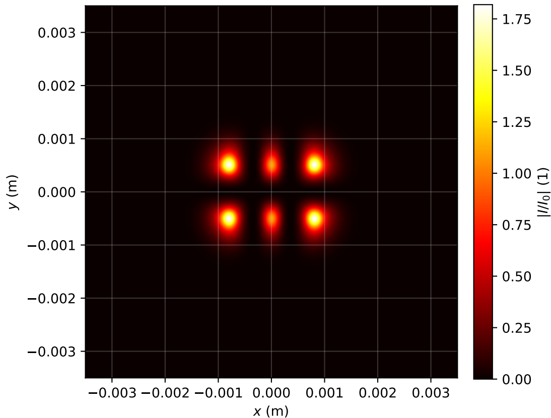
Intensity profile I(x, y, z = 0.318)/I_0 , \text{Pin}=6.0\text{Pcr} , artificial time
